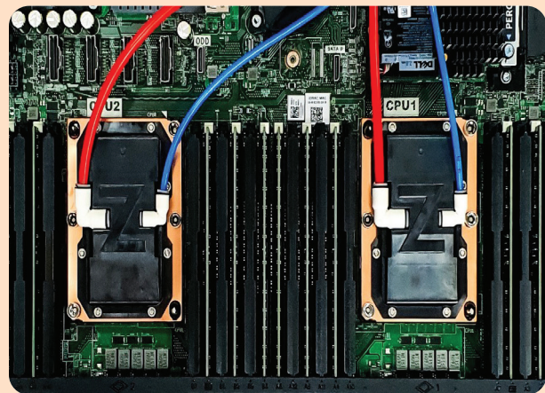
Figure 4 – Direct to Chip water-cooled plates
