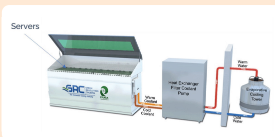
Figure 2 – Immersion Cooling
